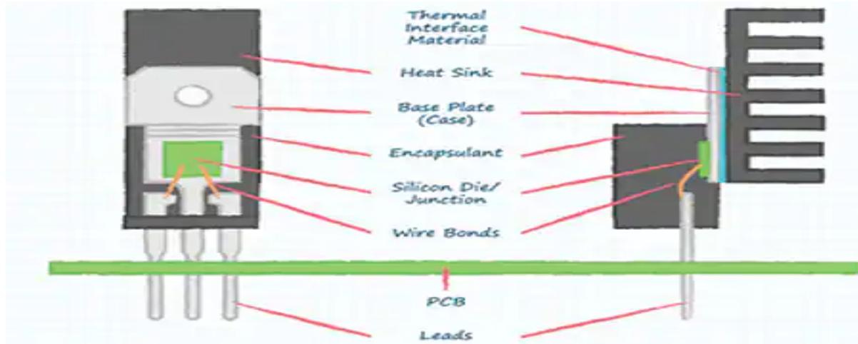
Figure 22: Heat Sink Attached to a Regulator
