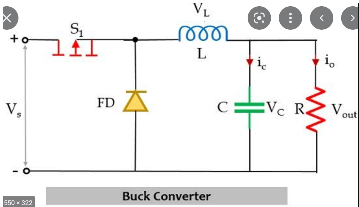
Figure 24: Buck Converter
