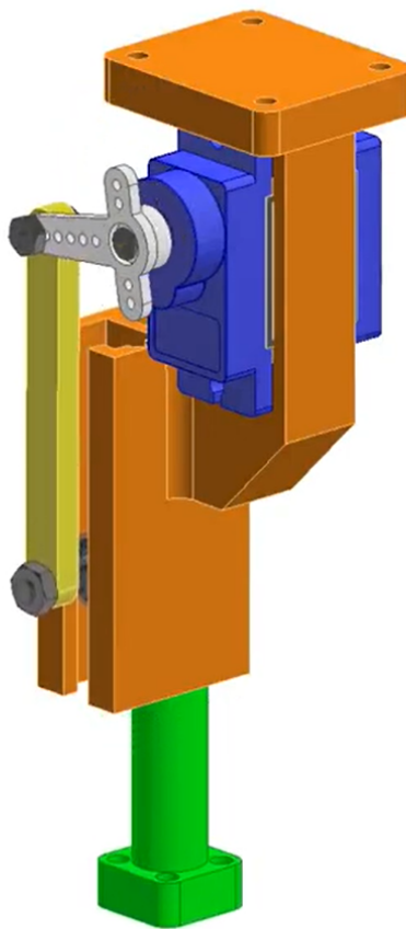
Figure 72: 3D-Printed Linear Actuator GrabCAD by Luca Delbarba Feb 28th 2022
