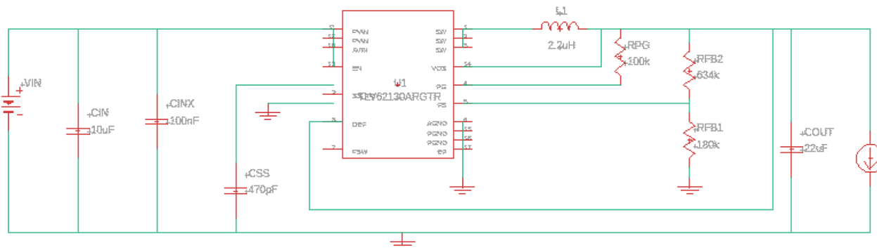
Figure 44: Voltage regulator for Microcontroller
