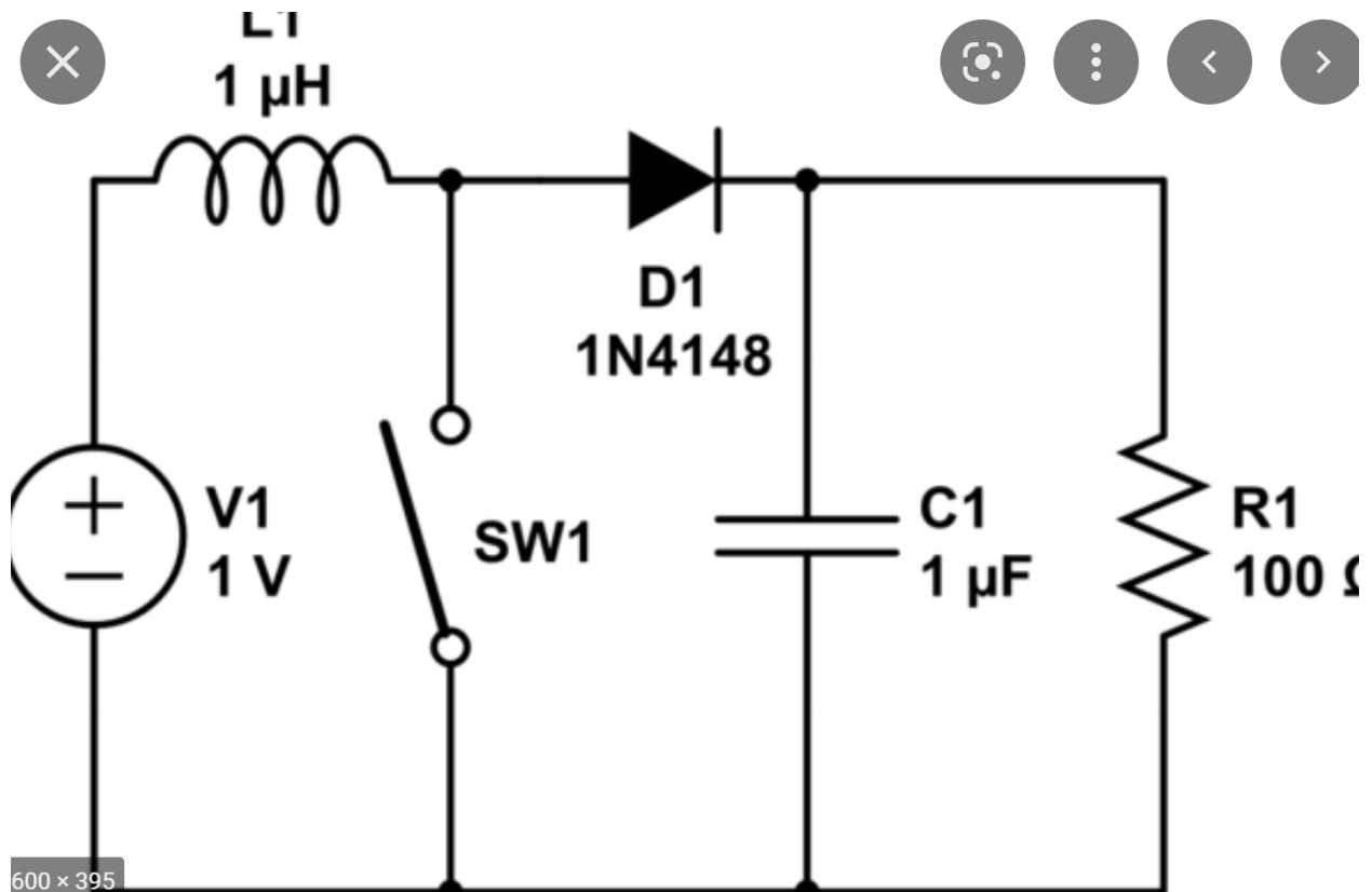
Figure 23: Boost Converter
