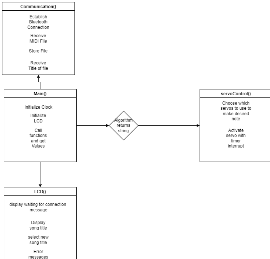
Figure 54: Microcontroller Code Block Diagram
