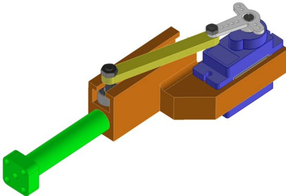
Figure 18: Assembly for conversion of rotational servo motion to linear actuation https://www.youtube.com/watch?v=MeLLaGI1es
